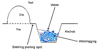
: Negarim water catchment
